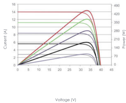
Current-Voltage & Power-Voltage Curves (435W)
